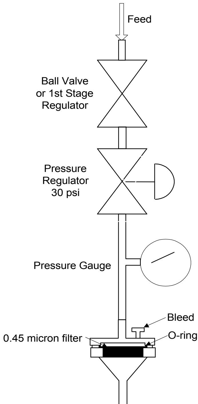
Figure 1. Apparatus
