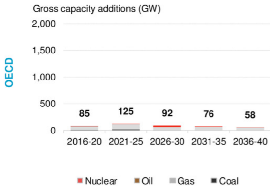
Figure 48: Gross five-year fossil-fuel and nuclear capacity additions
