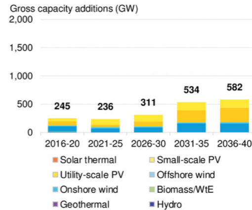
Figure 49: Gross five-year renewable capacity additions
