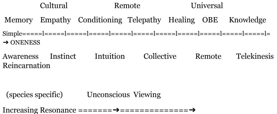
Figure 4. The spectrum of Quantum Hologram Resonance (Mitchell and Staretz, 2011).
