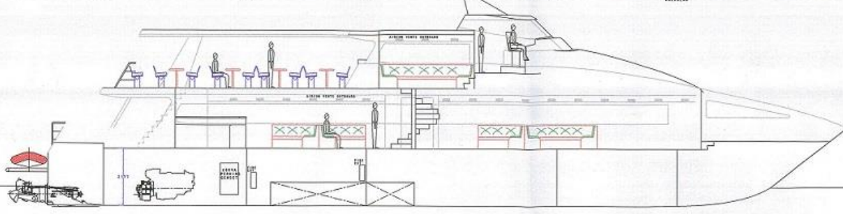
CENTRELINE PROFILE
