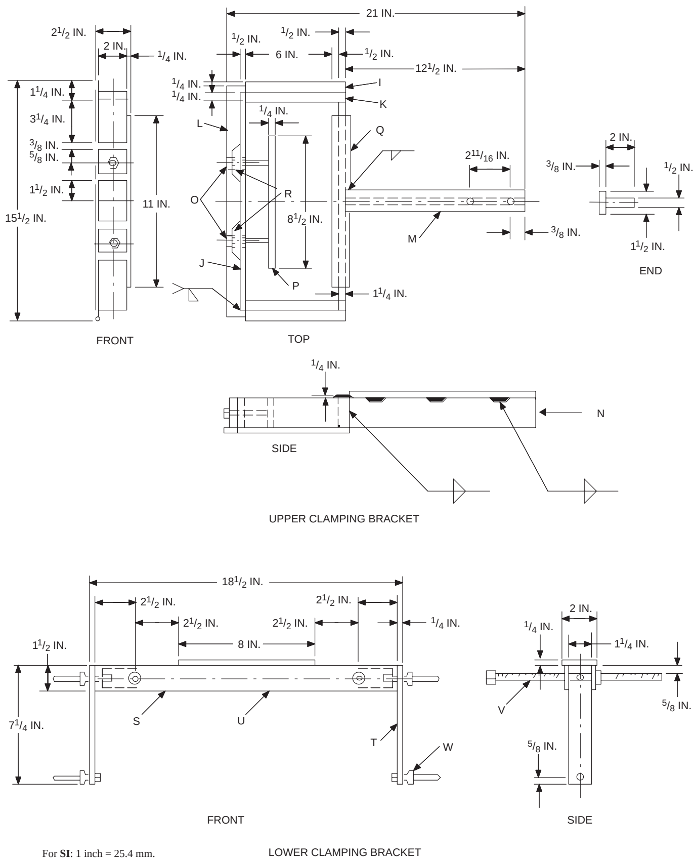
FIGURE 21-20-2—DETAIL DRAWINGS OF BOND WRENCH (Continued)
