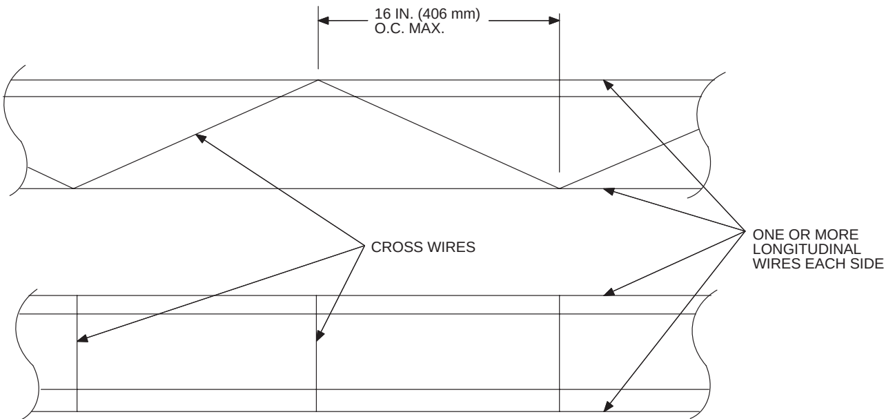
FIGURE 21-10-1—JOINT REINFORCEMENT
