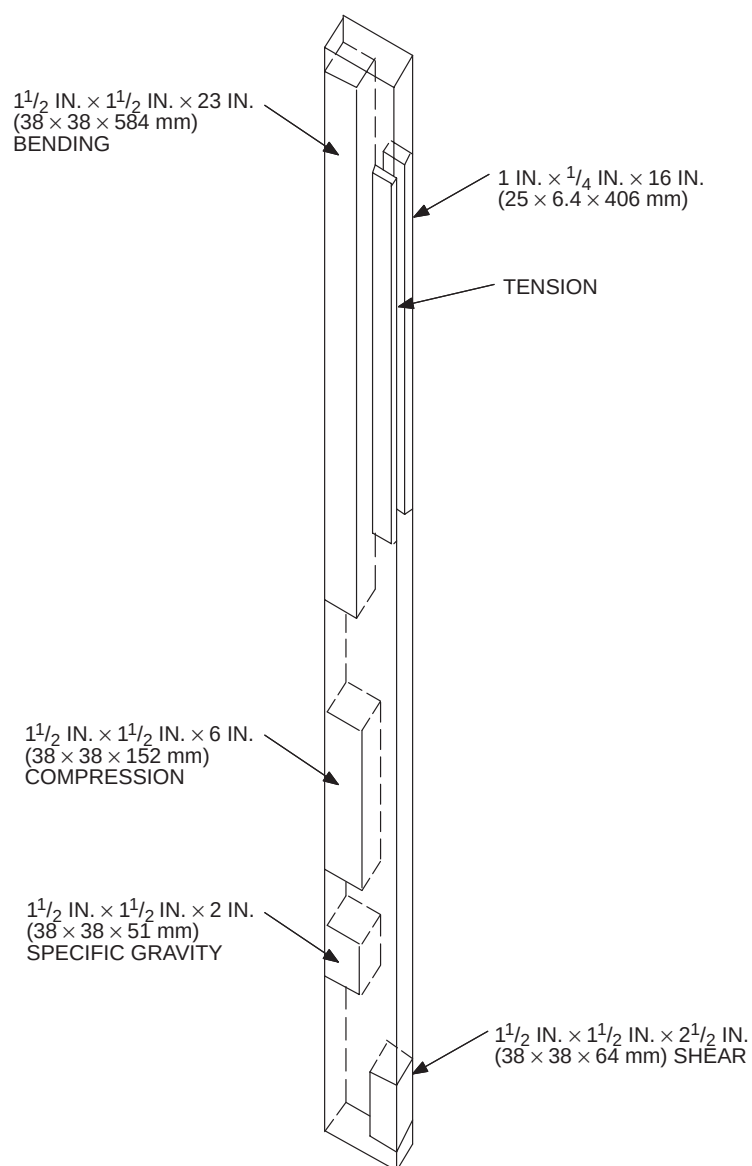
FIGURE 23-5-1—MATCHING DIAGRAM
