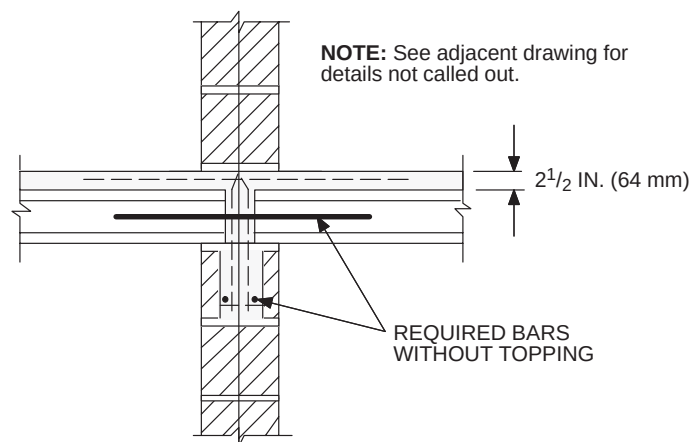
FIGURE A-21-13—VARIOUS TYPES OF WALL CONNECTIONS—(Continued)
