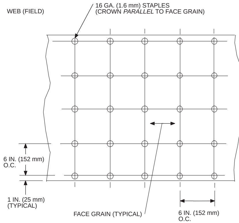
FIGURE 23-VI-1—STAPLE SPACING FOR PLYWOOD WEBS, FLANGES, SPLICE PLATES AND STIFFENERS
