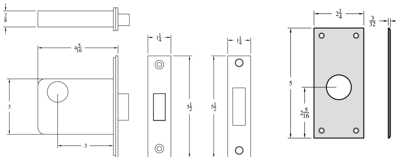
R278 ESCUTCHEON PLATE
