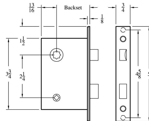
6539 Privacy Lock Dimensions
