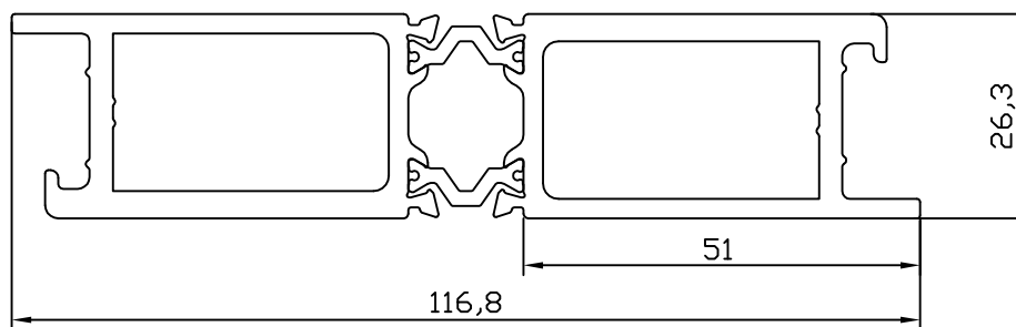
PREMARCO ALBA PROS 80RPT
