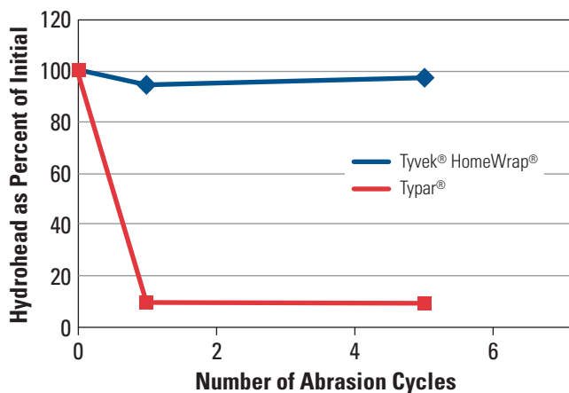
WATER RESISTANCE AFTER ABRASION (AATCC 127)
