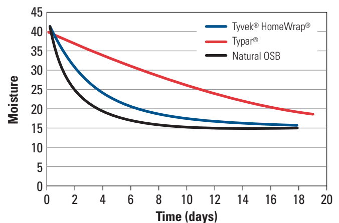
OSB DRYING CURVES (85°F / 80% RH)
