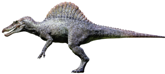
Spinosaurus
