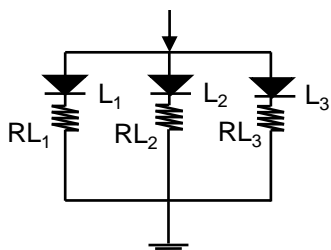
Fig.1. Recommended Circuit in Parallel Mode : Separate resistors must be used for each LED.
