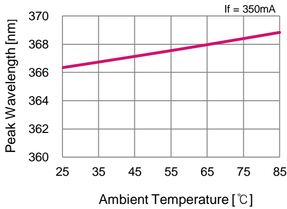
■ Ambient Temperature vs. Peak Wavelength
