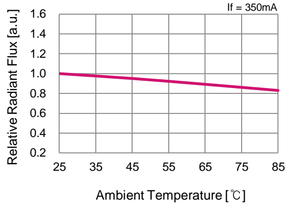
■ Ambient Temperature vs. Relative Radiant Flux
