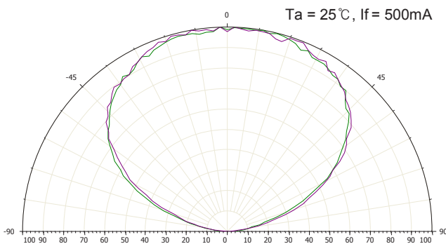
■ Radiation Characteristics
