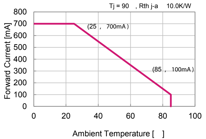
Derating Curve
