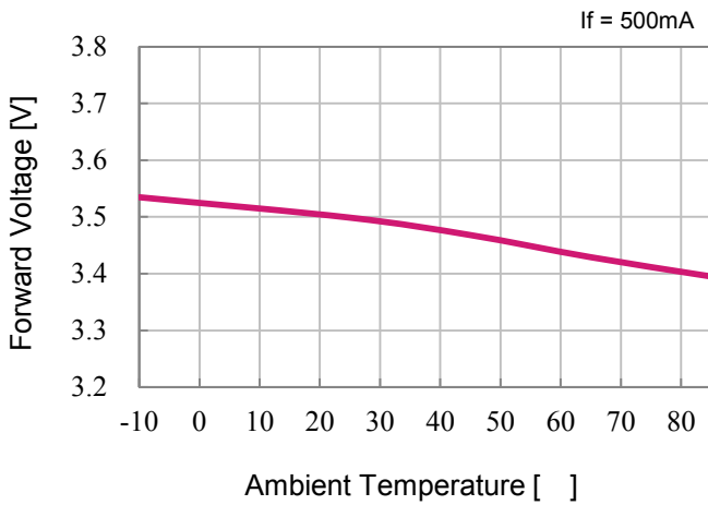
Ambient Temperature vs. Forward Voltage
