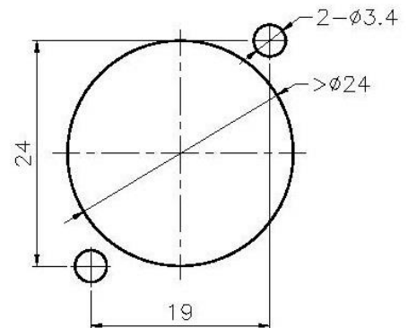
Panel Cutout
