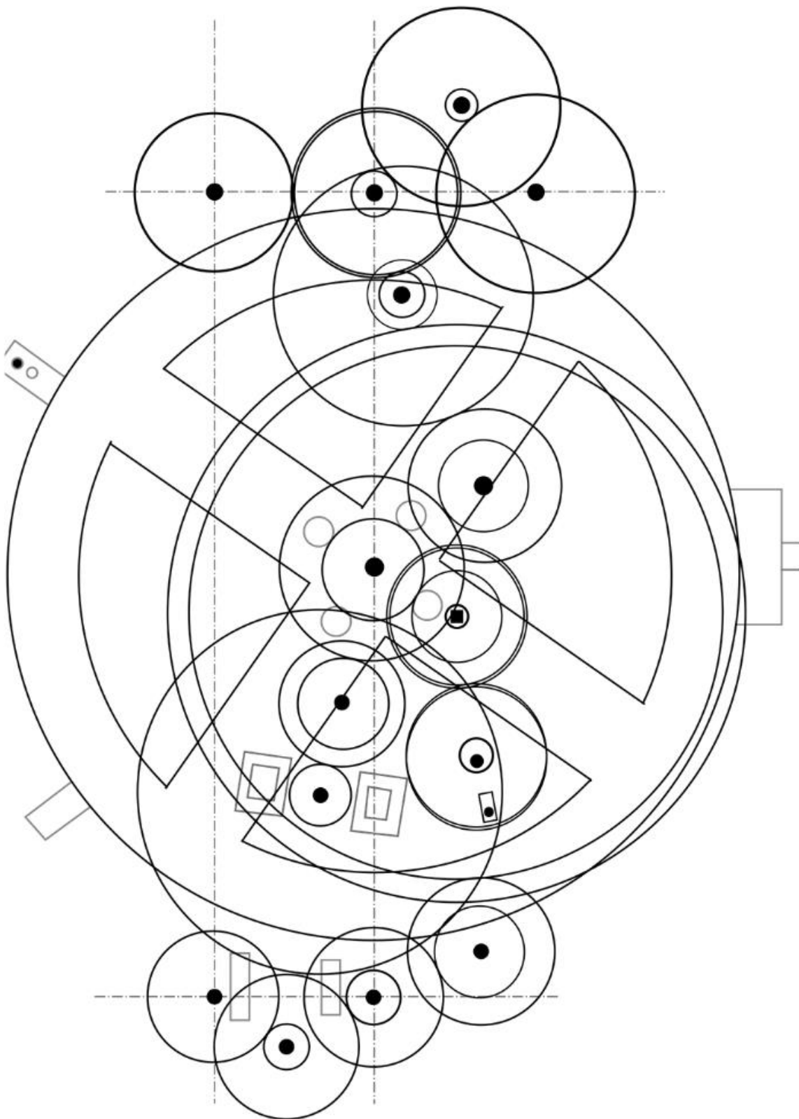
Antikythera Mechanism: Schematic
