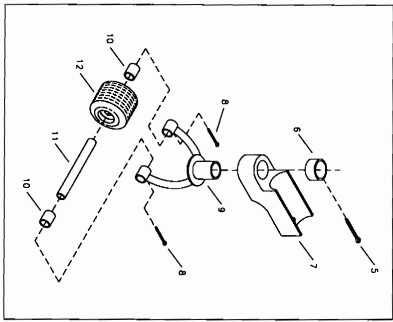
TAILWHEEL ASSEMBLY DETAIL
