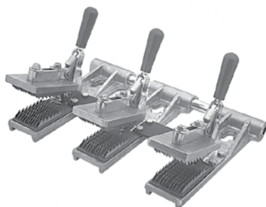
Triple Lockjaws #203
