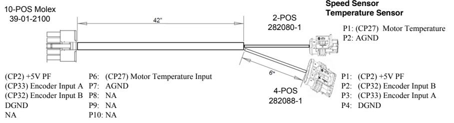
Navitas PN: 40-000580 AC Motor Adapter for 10-000726 Motor
