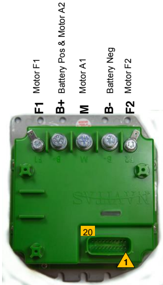
Navitas TSX DC Shunt Controller
