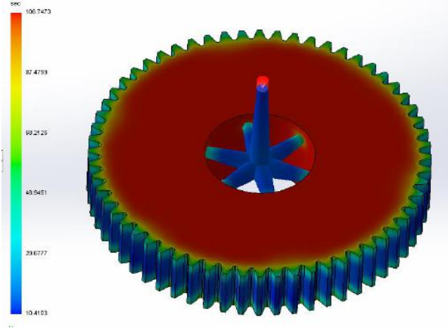
Figure 12. Cooling time simulation
