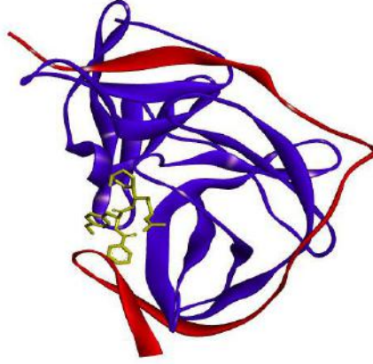
Şekil 3. 5LC0 proteininin A zinciri. NS2B kırmızı, NS3 mavi, ligand (N-((S)-3-(4-(aminomethyl)phenyl)-1-(((R)-4-guanidino-1-(5-hydroxy-1,3,2-dioxaborinan-2-yl)butyl)amino)-1-oxopropan-2-yl)benzamide- 6T8) molekülü ise sarı renkle gösterilmiştir.
