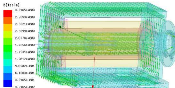
Figure 4. Flux density and flux lines of the proposed EVS.
