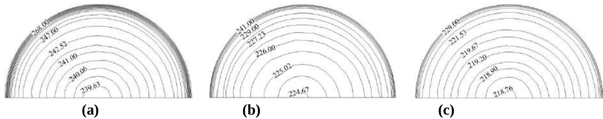
Figure 6. Temperature distributions of \text{TiO}_2/\text{R134a} nanorefrigerant at the outlet of the duct for different Reynolds numbers: (a) \text{Re}=3000 , (b) \text{Re}=6000 , (c) \text{Re}=10000
