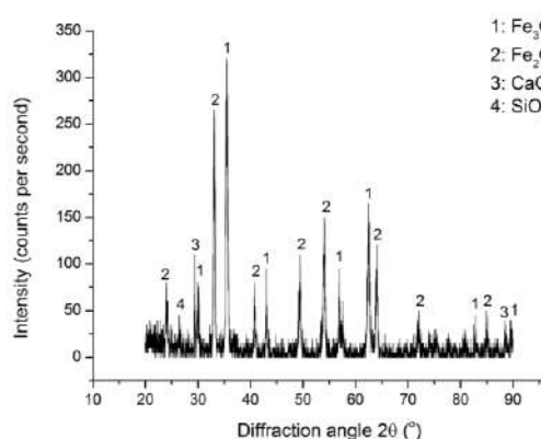
Figure 4. XRD image of enriched ore in -45 \mu\text{m} grain size.
