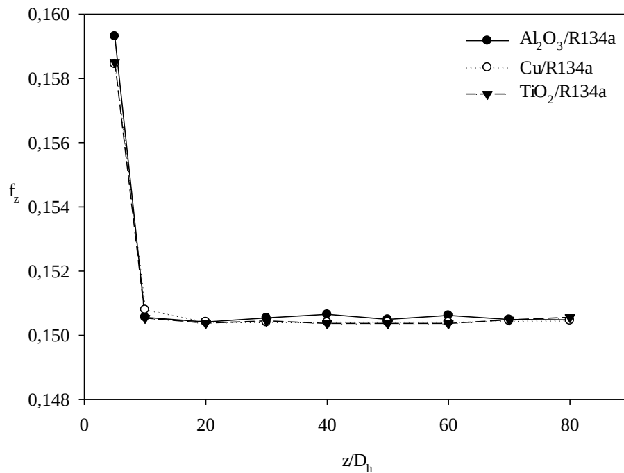
Figure 12. The changing of (a) local heat transfer coefficient and (b) local Darcy friction factor through the duct length for different nanorefrigerant types
