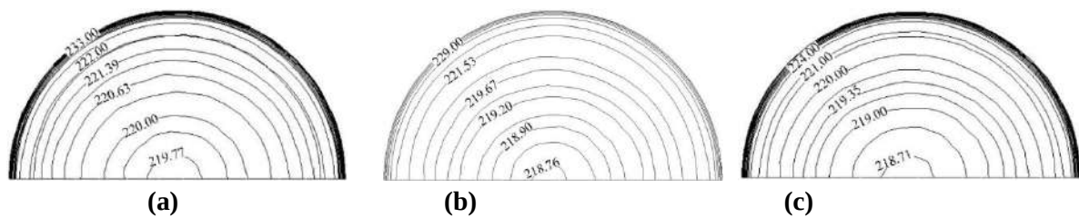
Figure 10. Temperature distributions of different types of nanorefrigerants at the outlet of the duct: (a) Cu/R134a, (b) TiO_2/R134a , (c) Al_2O_3/R134a
