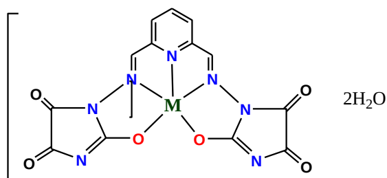
Figure 1. Proposed structure of Cu(II), Ni(II) and Co(II) complexes.
