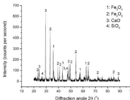
Figure 2. XRD analysis of the ore
