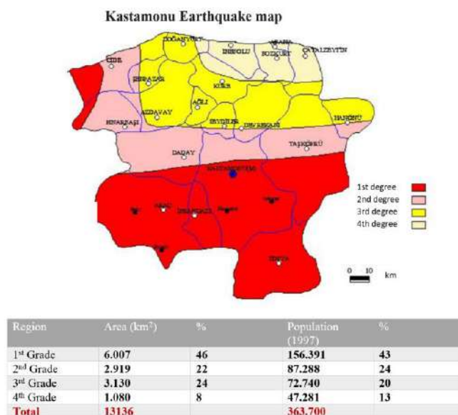
Figure 1. Kastamonu earthquake map
