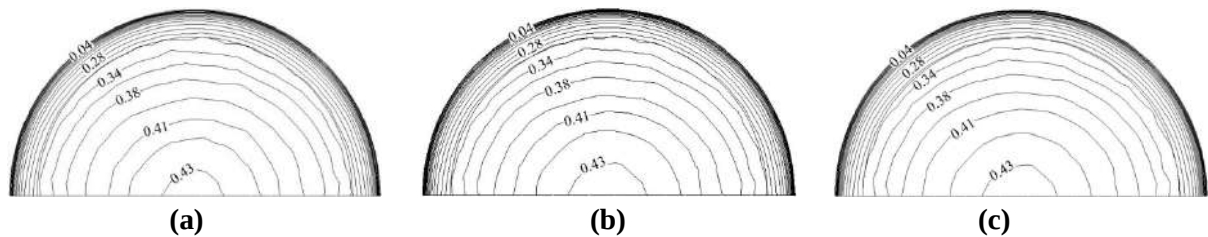
Figure 7. Velocity distributions of \text{TiO}_2/\text{R134a} nanorefrigerant at the outlet of the duct for different nanoparticle volume fractions: (a) \phi=0.8\% , (b) \phi=2.0\% , (c) \phi=4.0\%
