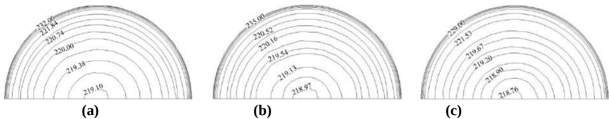
Figure 8. Temperature distributions of \text{TiO}_2/\text{R134a} nanorefrigerant at the outlet of the duct for different nanoparticle volume fractions: (a) \phi=0.8\% , (b) \phi=2.0\% , (c) \phi=4.0\%
