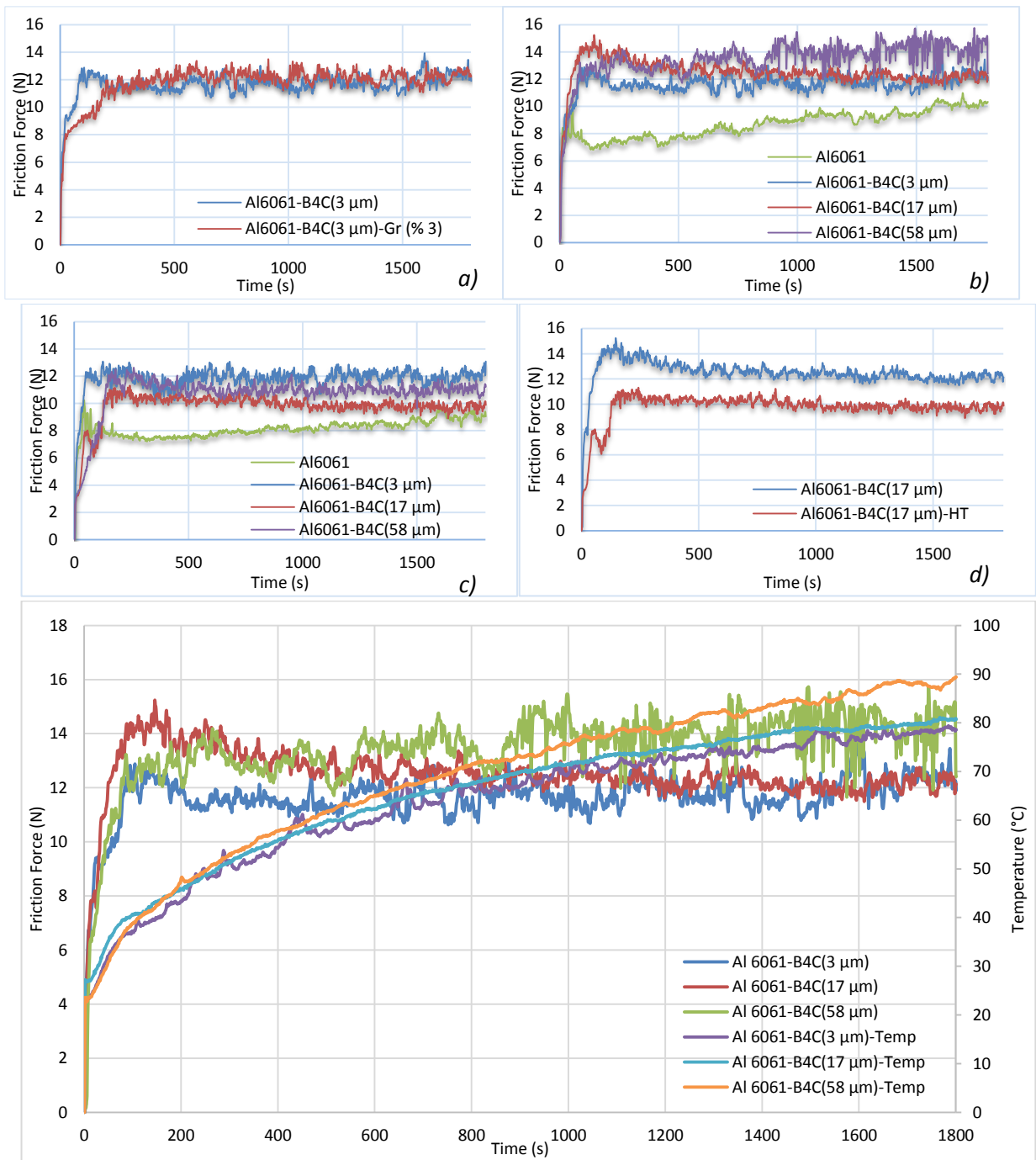
Figure 5. Friction forces of samples a) Friction forces of Al 6061-B4C(3 \mu\text{m} ) and Al 6061-B4C(3 \mu\text{m} )-Gr samples b) Friction forces of Al 6061, Al 6061-B4C(3 \mu\text{m} ), Al 6061-B4C(17 \mu\text{m} ) and Al 6061-B4C(58 \mu\text{m} ) samples without heat treatment c) Friction forces of Al 6061, Al 6061-B4C(3 \mu\text{m} ), Al 6061-B4C(17 \mu\text{m} ) and Al 6061-B4C(58 \mu\text{m} ) samples with heat treatment d) Friction forces of Al 6061-B4C(17 \mu\text{m} ) with and without heat treatment e) Friction forces and temperature values of Al 6061-B4C(3 \mu\text{m} ), Al 6061-B4C(17 \mu\text{m} ) and Al 6061-B4C(58 \mu\text{m} ) samples without heat treatment
