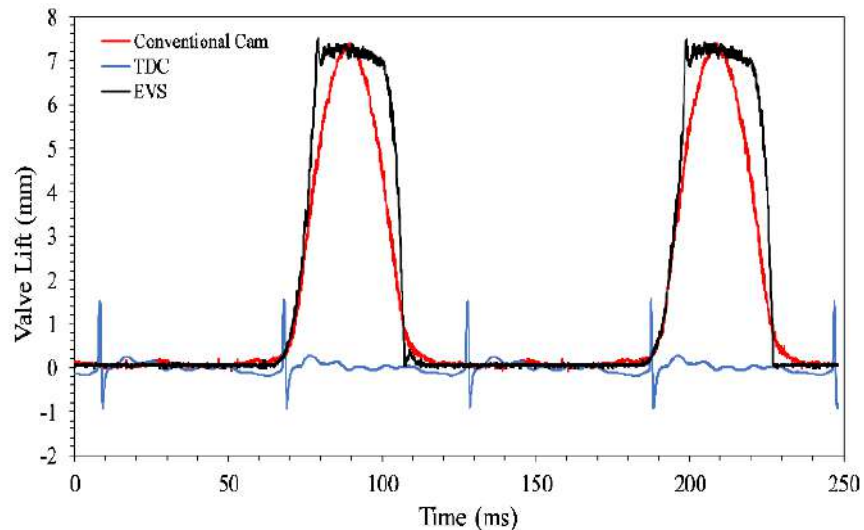
Figure 8. Conventional and EVS valve profile
