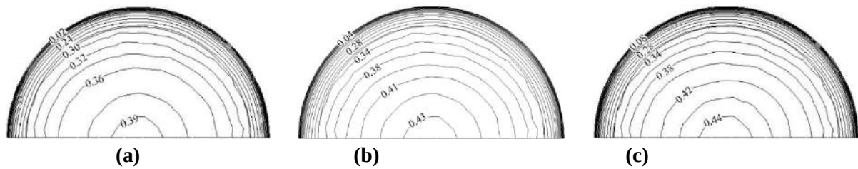
Figure 9. Velocity distributions of different types of nanorefrigerants at the outlet of the duct: (a) Cu/R134a, (b) TiO_2/R134a , (c) Al_2O_3/R134a
