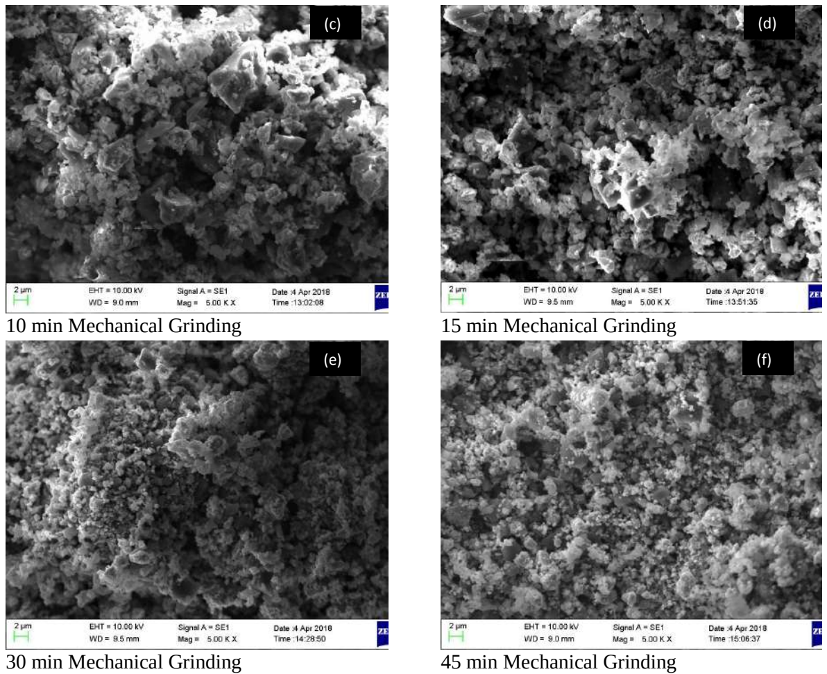
Figure 6. SEM images of samples subjected to mechanical grinding at different times with the original mixture.
