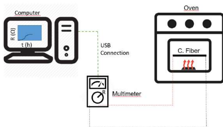
Figure 1. The thermal aging setup of CF
