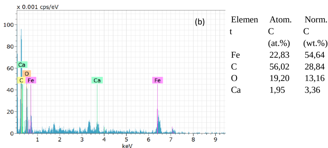
Figure 5. (a) SEM image (500X), (b) EDX analysis of the original mixture of -45\ \mu\text{m} size prepared to be 2 times the stoichiometric ratio.
