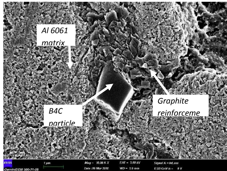
Figure 7. Microstructure of Al 6061-B4C (3 \mu\text{m} )-Gr sample.
