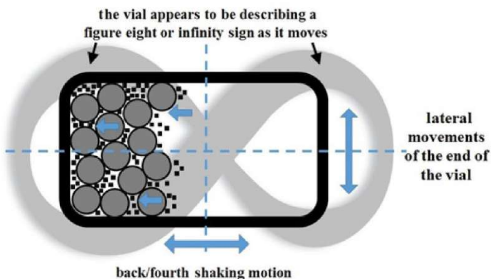
Figure 8. Working principle of spex type mill used in grinding [20].
