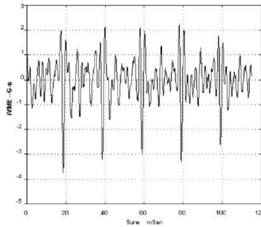
Figure 13. Looseness wave form graphs [13]
