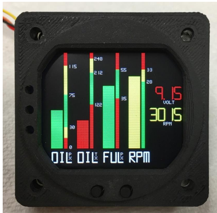
Engine monitor. Note color coding. System voltage is red when below 12.00 volts
