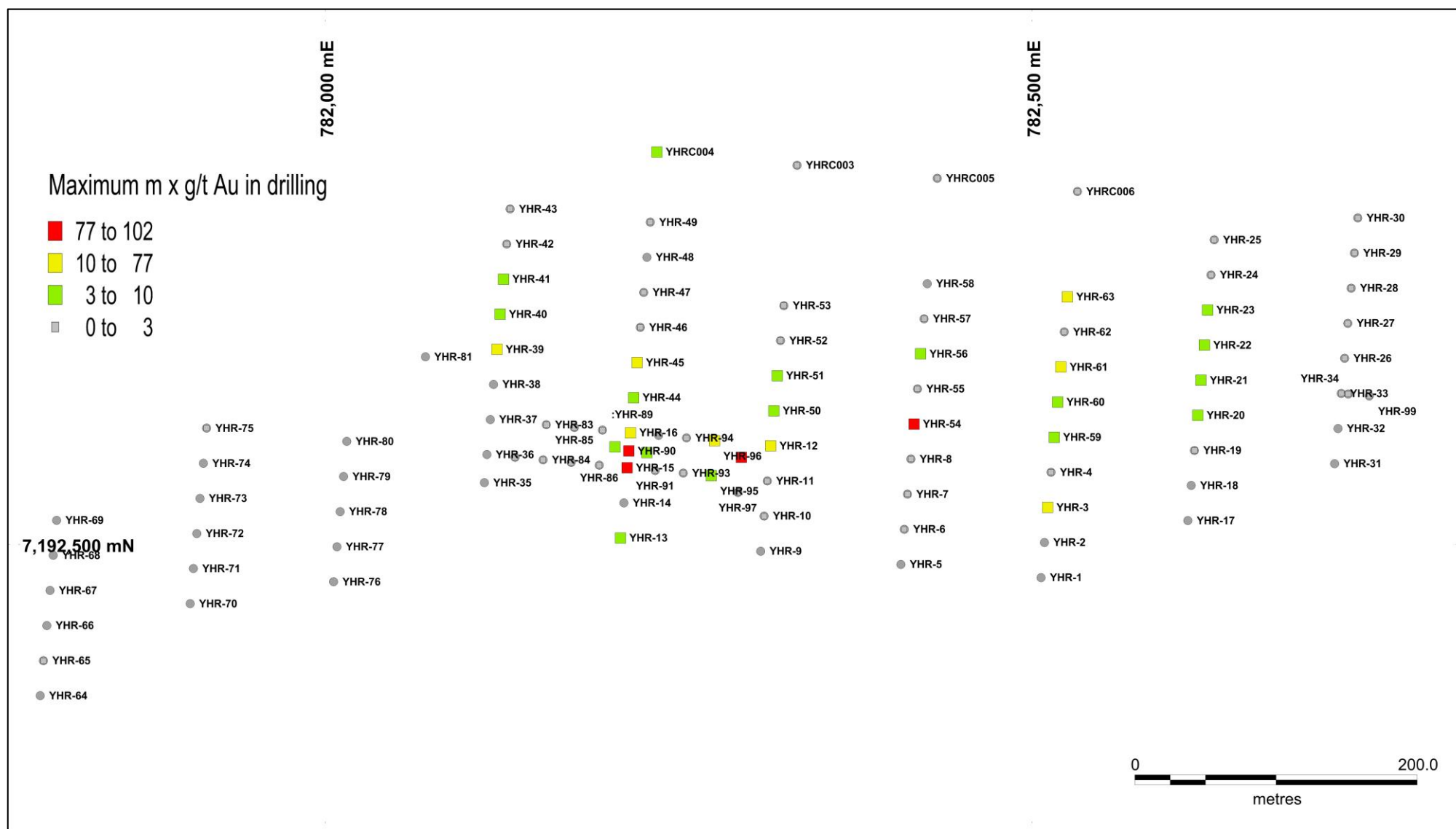
Figure 4 Boundary Fence prospect drill collar plan showing historic intersections as metres x g/t gold (GDA94 Zone 50, re-projected from local grid).
