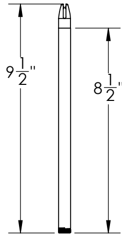
03-1229-23 9" Spreader Tube Threaded
