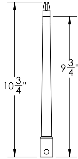
03-1248-23 9" Spreader Tube
