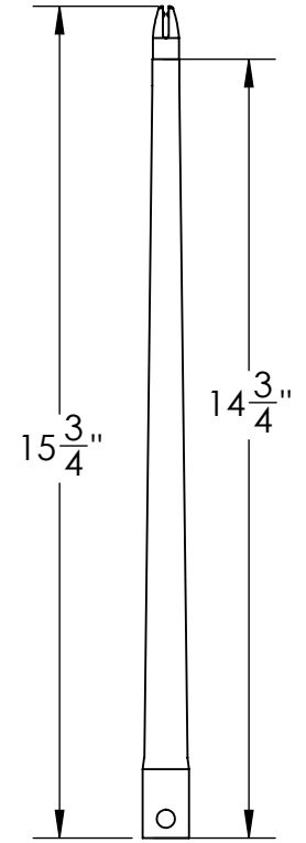
03-1250-23 15" Spreader Tube
