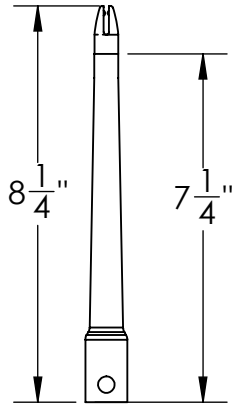
03-1247-23 7" Spreader Tube
