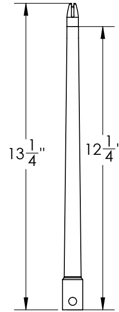
03-1249-23 12" Spreader Tube
