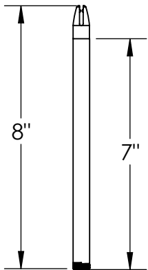
03-1229-23- MOD 7" Spreader Tube Threaded
