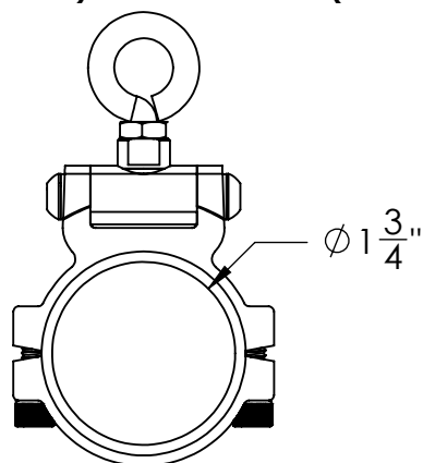
03-1856-23T 1 3/4" Teaser Clamp Tournament Outrigger Lower Intermediate Tube (Above 1st Spreader)
