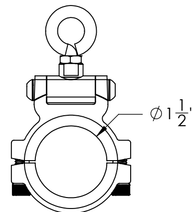
03-1856-TSM 1 1/2" Teaser Clamp Carbon Fiber 22' Pole (Above Base Tube)
