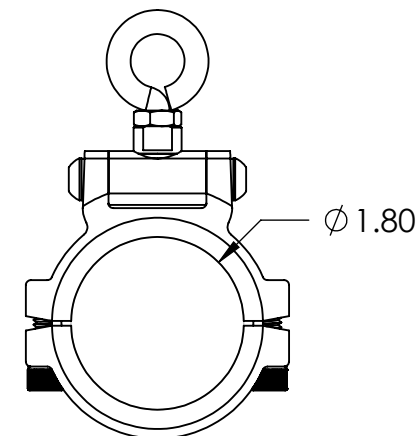
03-1154-23TS 1.8" Teaser Clamp Carbon Fiber 22' Pole (Base Tube)
