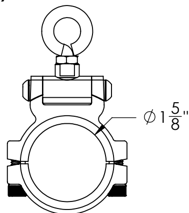
03-1856-TS 1 5/8" Teaser Clamp Tournament Outrigger Upper Intermediate Tube (Above 2nd Spreader)
