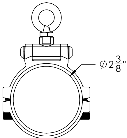
03-1531-23T 2 3/8" Teaser Clamp Bigg Rigg Outrigger Main Base tube (Below 1st Spreader)
