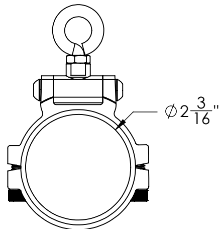
03-1528-23T 2 3/16" Teaser Clamp Bigg Rigg Outrigger Lower Intermediate Tube (Above 1st Spreader)
