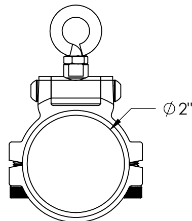
03-1154-23T 2" Teaser Clamp Tournament Outrigger Main Base Tube (Below 1st Spreader)
