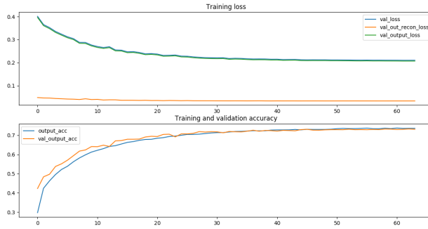
Figure 9. Loss and Accuracy Curve
