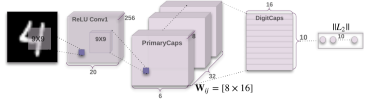
Figure 1. Architecture of Capsule Networks
