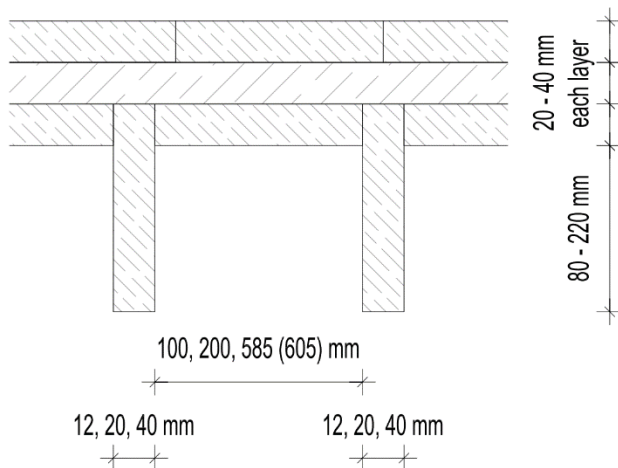
Figure 4: The ribbed-Xlam plate geometries selected for further production development and testing
