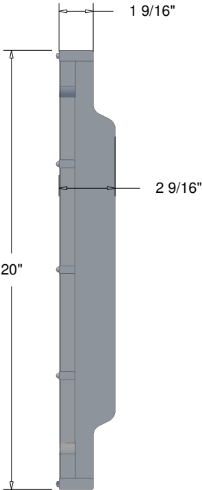
END VIEW
