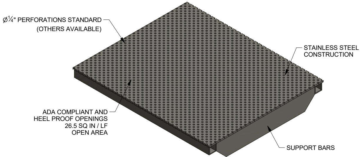
ISOMETRIC VIEW
