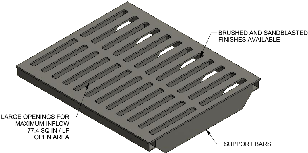
ISOMETRIC VIEW
