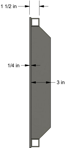
END VIEW
