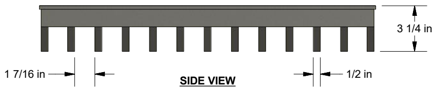
SIDE VIEW
