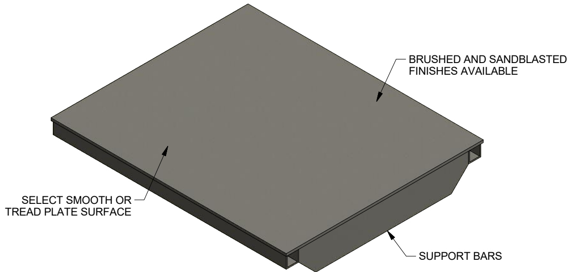
ISOMETRIC VIEW
