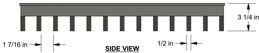
SIDE VIEW
