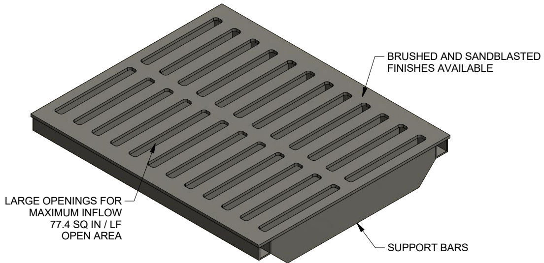
ISOMETRIC VIEW
