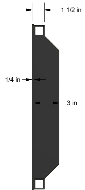
END VIEW
