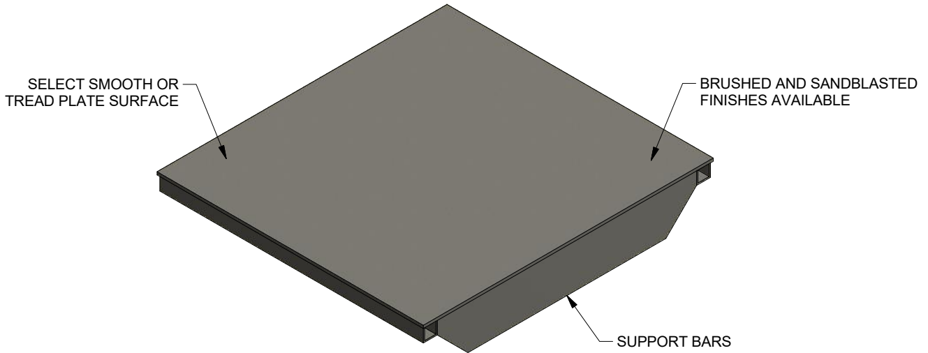
ISOMETRIC VIEW
