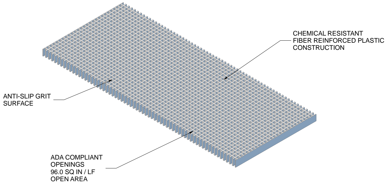
ISOMETRIC VIEW
