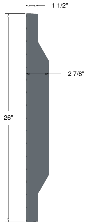
END VIEW
