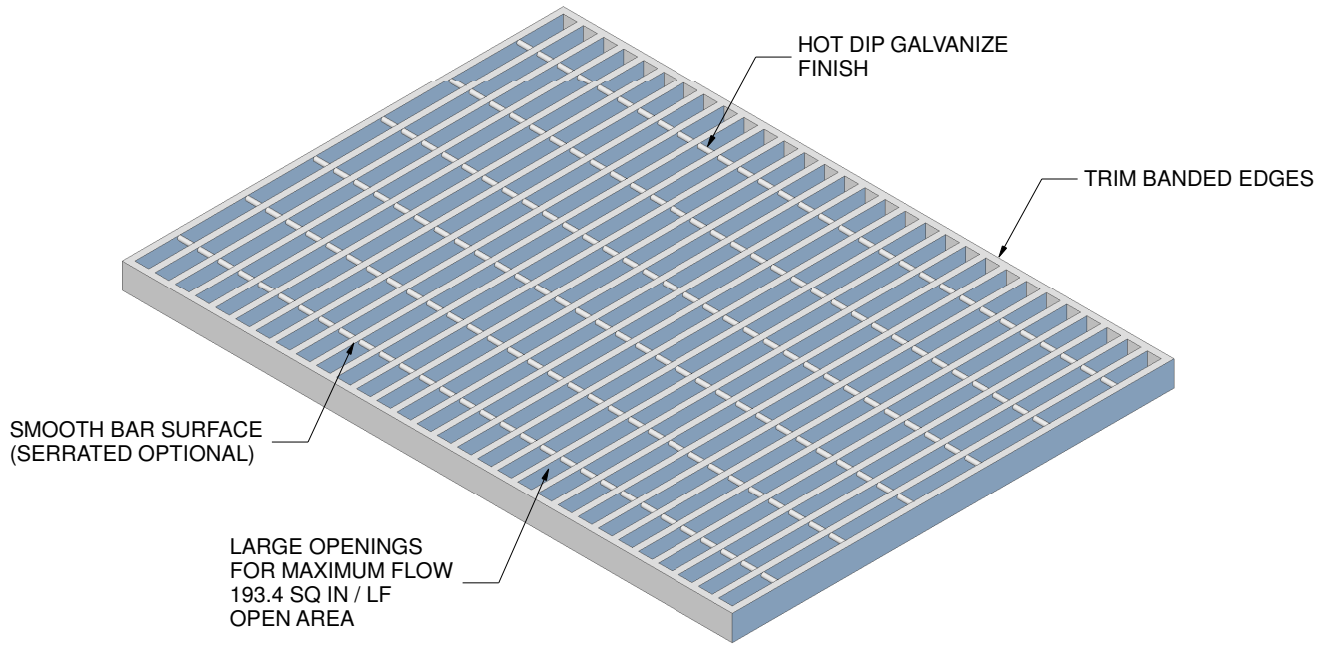
ISOMETRIC VIEW
