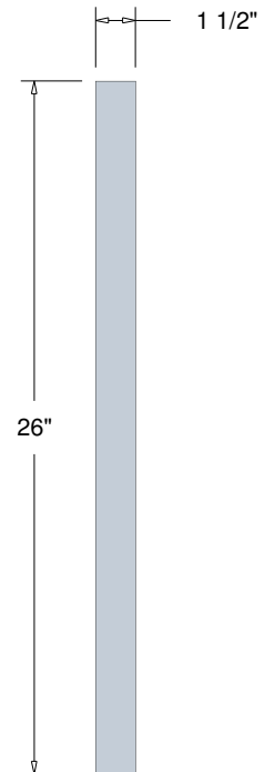
END VIEW
