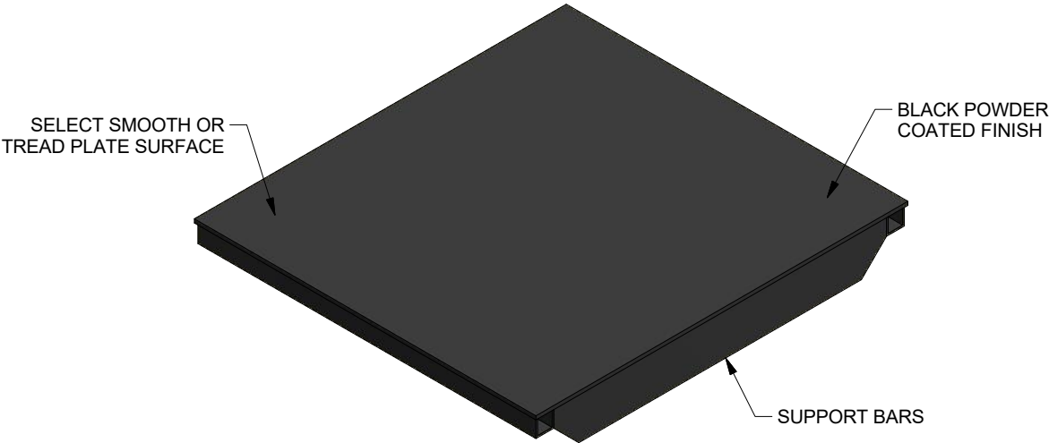
ISOMETRIC VIEW
