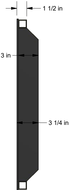
END VIEW
