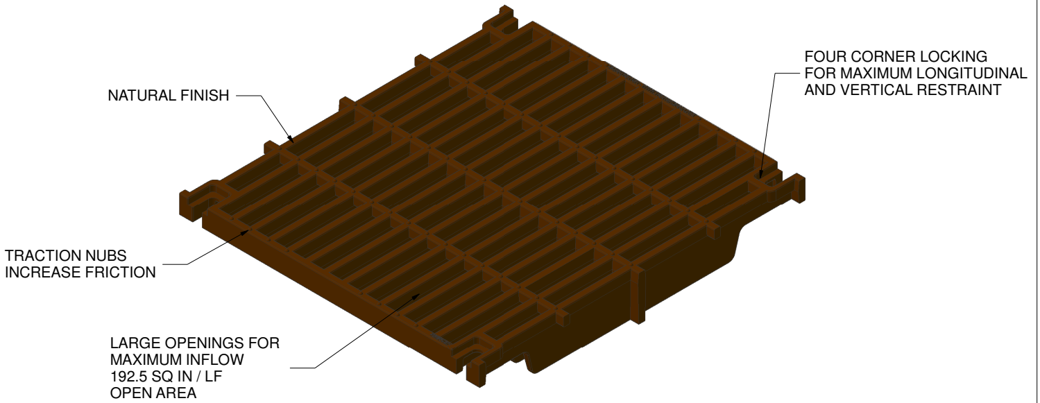
ISOMETRIC VIEW
