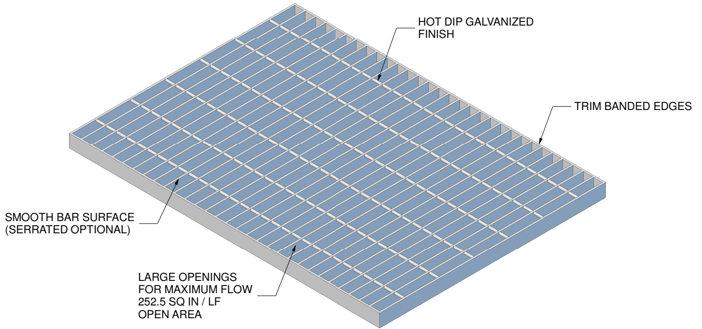
ISOMETRIC VIEW
