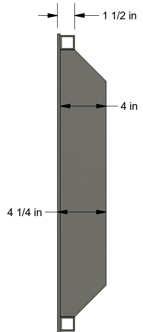
END VIEW
