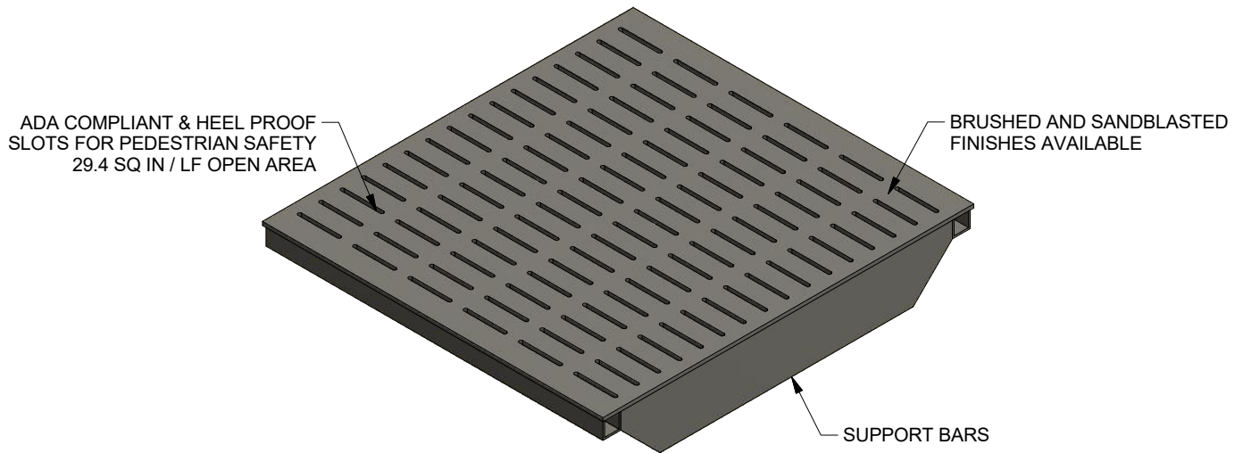
ISOMETRIC VIEW
