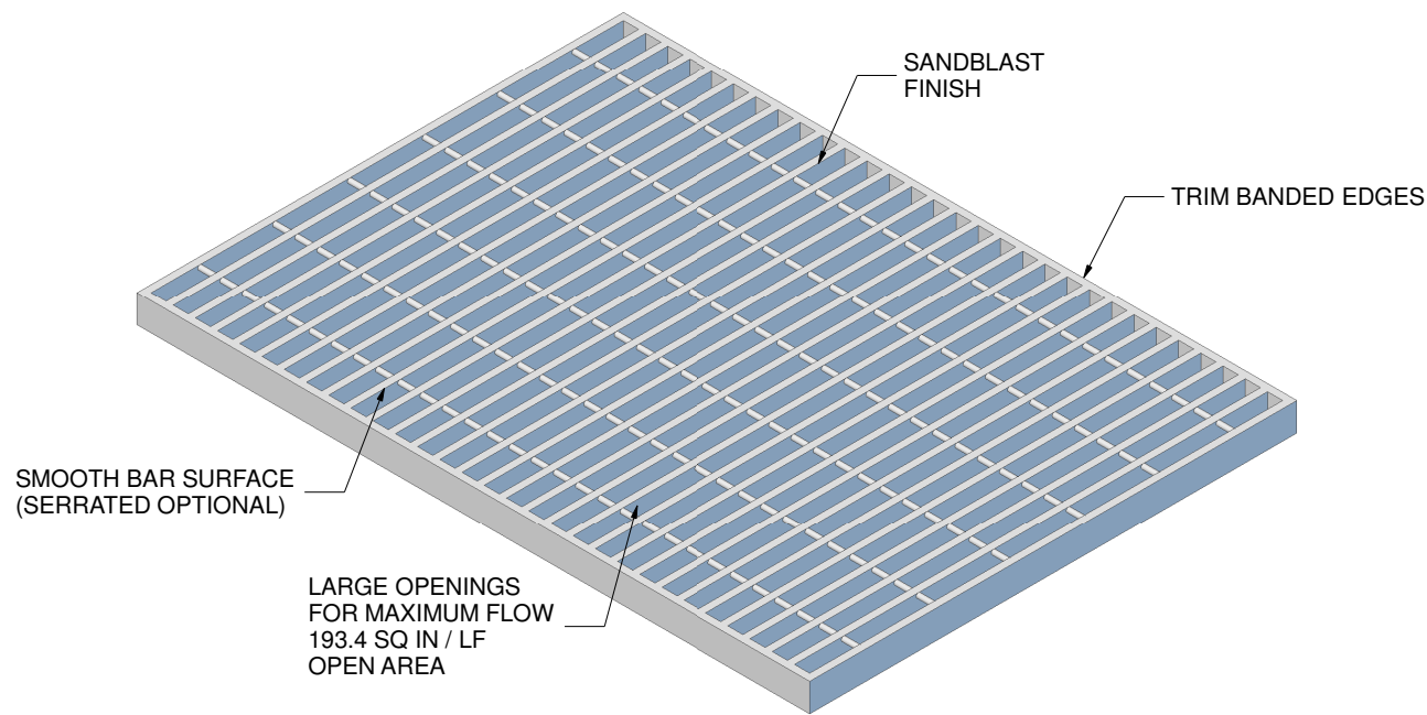
ISOMETRIC VIEW
