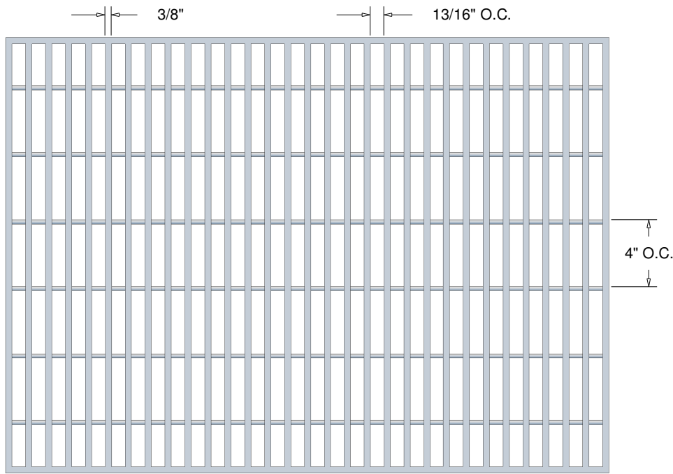
TOP VIEW
