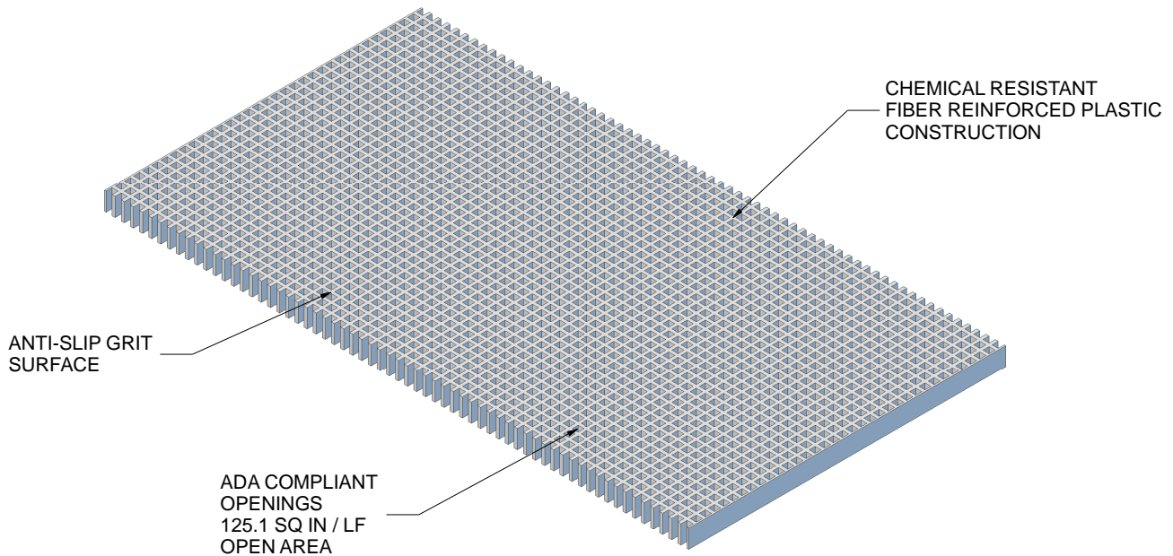
ISOMETRIC VIEW
