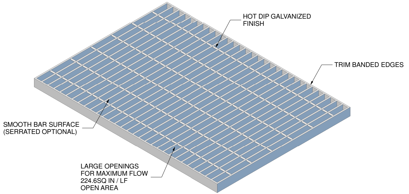
ISOMETRIC VIEW
