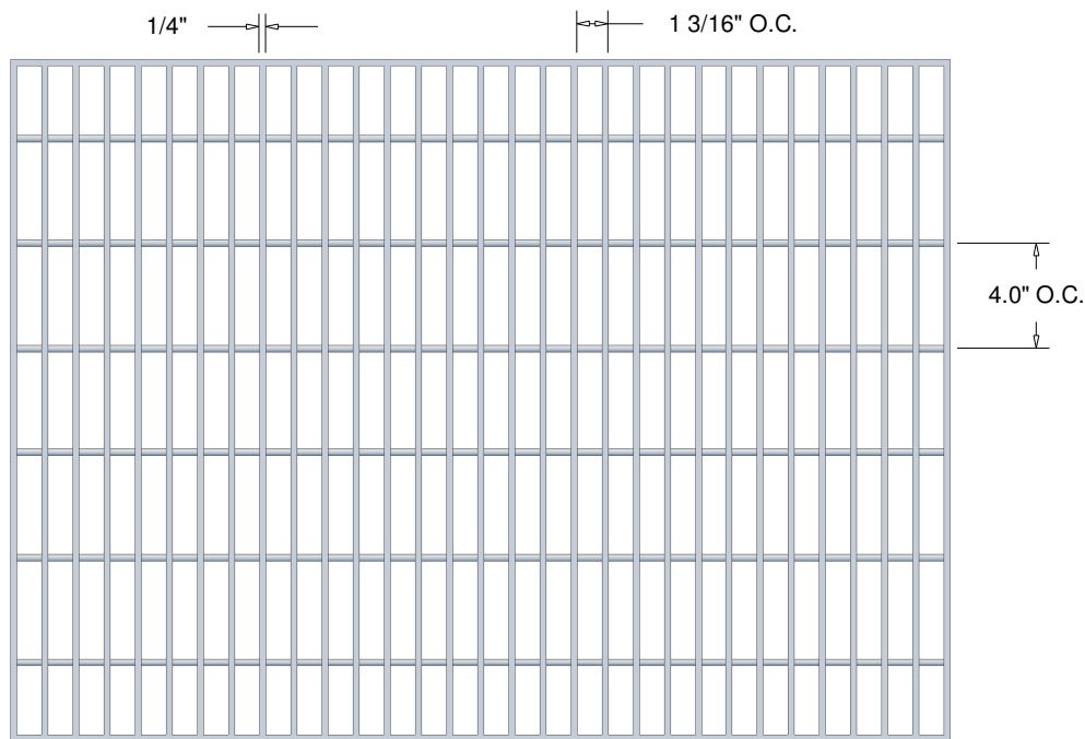
TOP VIEW
