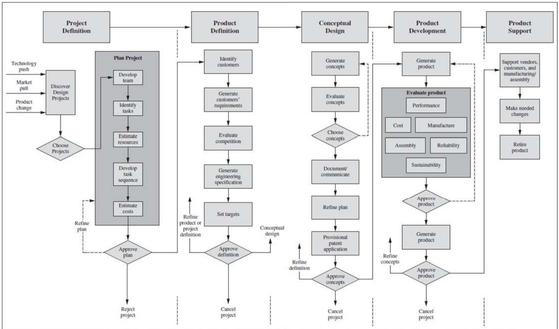
An overview of the mechanical design and product support process, Figure 4.5 in The Mechanical Design Process , Copyright David G. Ullman
