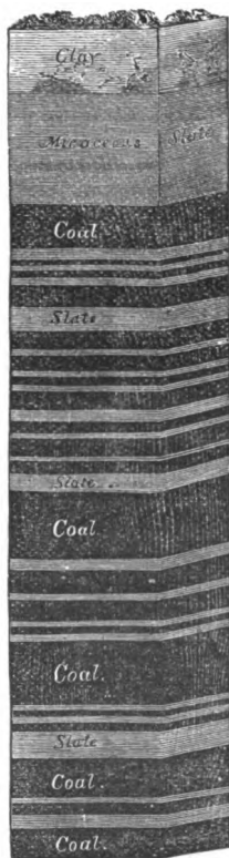
COAL-MEASURES OF PENN- SYLVANIA.
