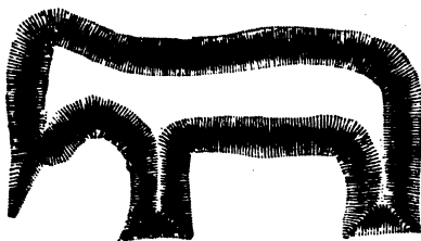
ELEPHANT MOUND, WISCONSIN.
