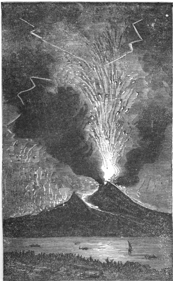
ERUPTION OF VESUVIUS IN 1737.
