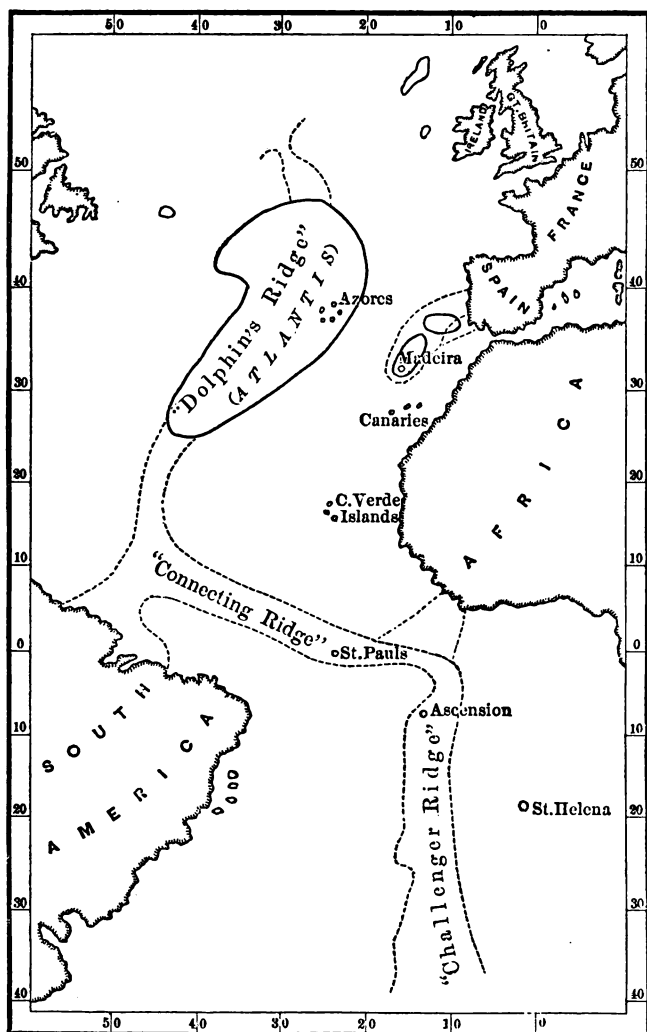
MAP OF ATLANTIC, WITH ITS ISLANDS AND CONNECTING RIDGES, FROM DEEP-SEA SOUNDINGS.
