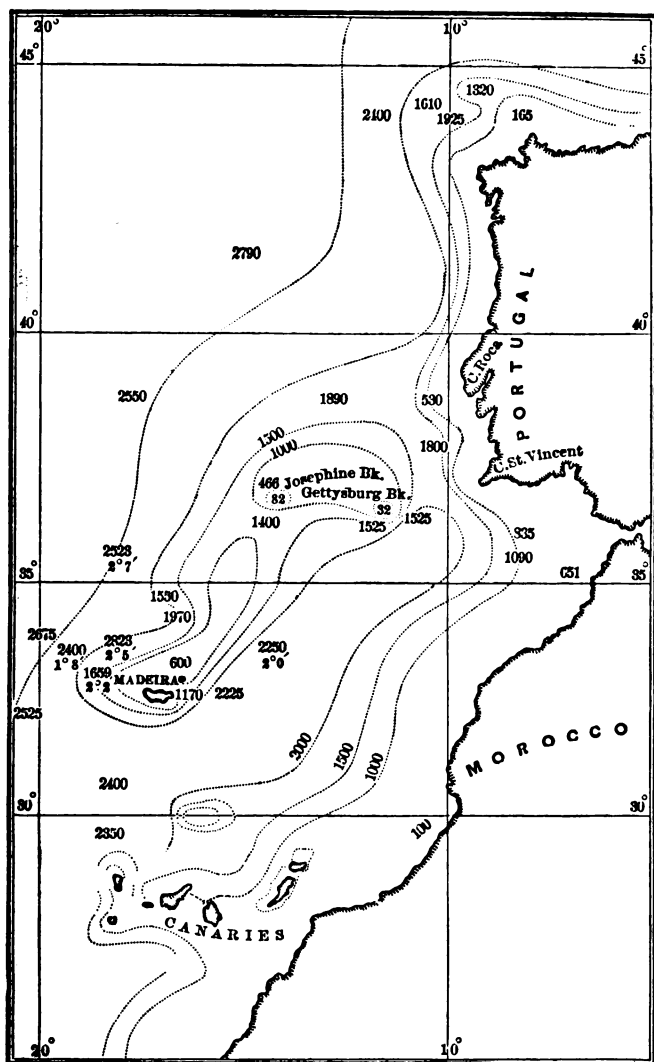
ANCIENT ISLANDS BETWEEN ATLANTIS AND THE MEDITERRANEAN, FROM DEEP-SEA SOUNDINGS.
