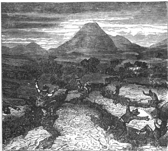
CALABRIAN PEASANTS INGULFED BY CREVASSES (1783).
