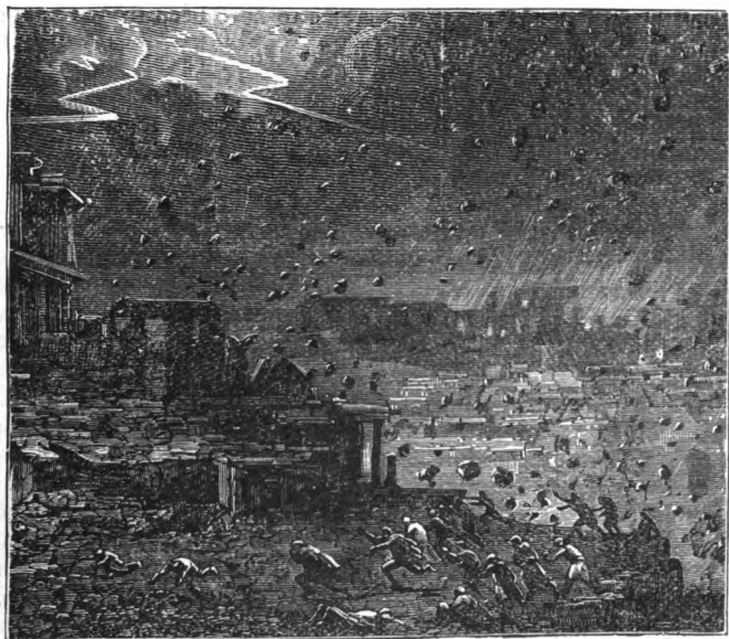
DESTRUCTION OF POMPEII.
