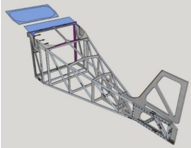
2: Rear Fuselage
