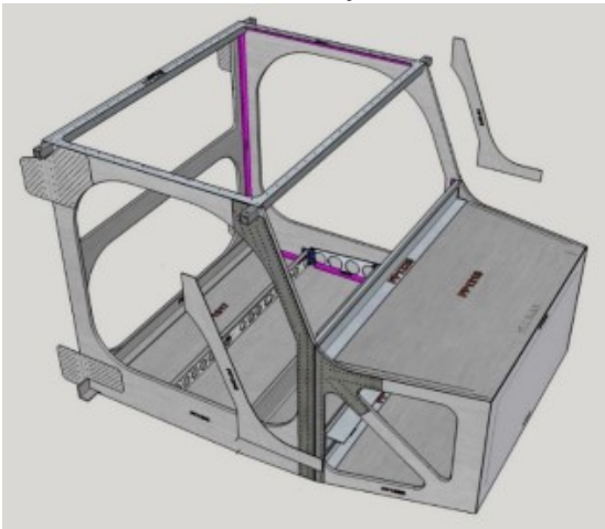
1: Cabin
