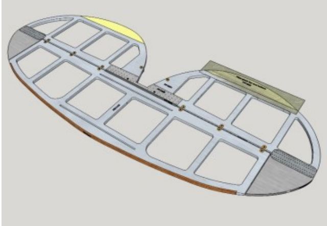
5: Horizontal surfaces
