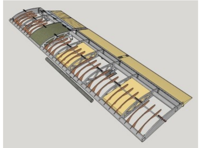
3: Wing
