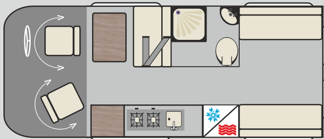
Aurora daytime
