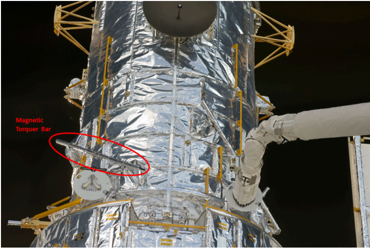
fig(1) Magnetorquer on the Hubble Telescope
